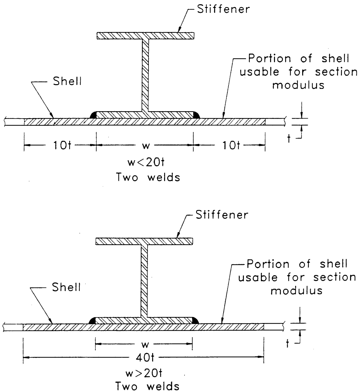
Figure 24. Definition of cross section for computation of section modulus of ring stiffener for DOT (non-ASME) tanks.
